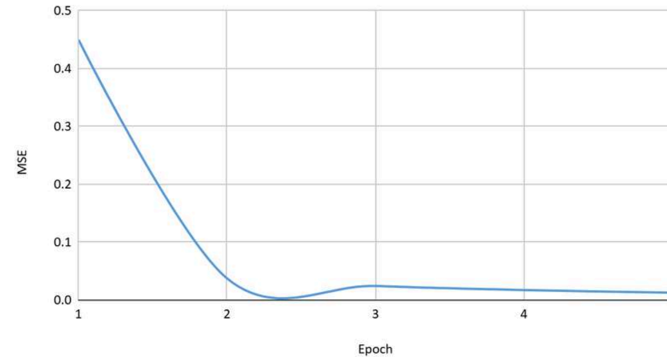
Chart MSE Training
